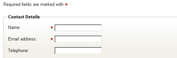
Figure 5.26: Required fields marked with absolutely positioned image of a star, aligned against form elements
